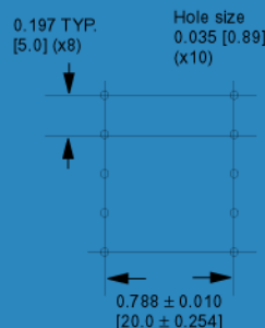
PCB Layout (Top)
