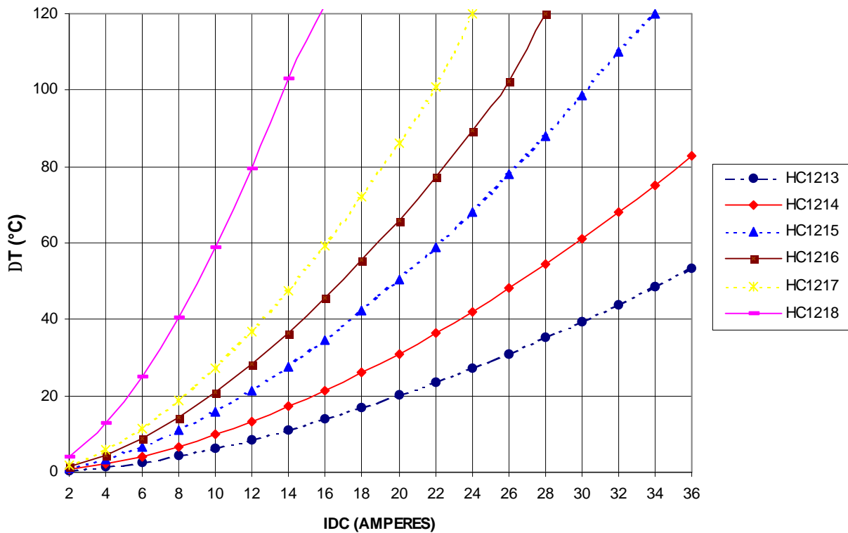
TEMPERATURE RISE vs CURRENT
